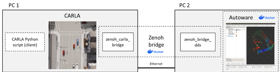
Figure 44: CAM research platform setup with a single AUTOWARE instance.
