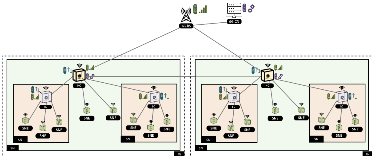
Figure 40: Subnetwork Architecture of the Inter-subnetwork Coordination Use Case
