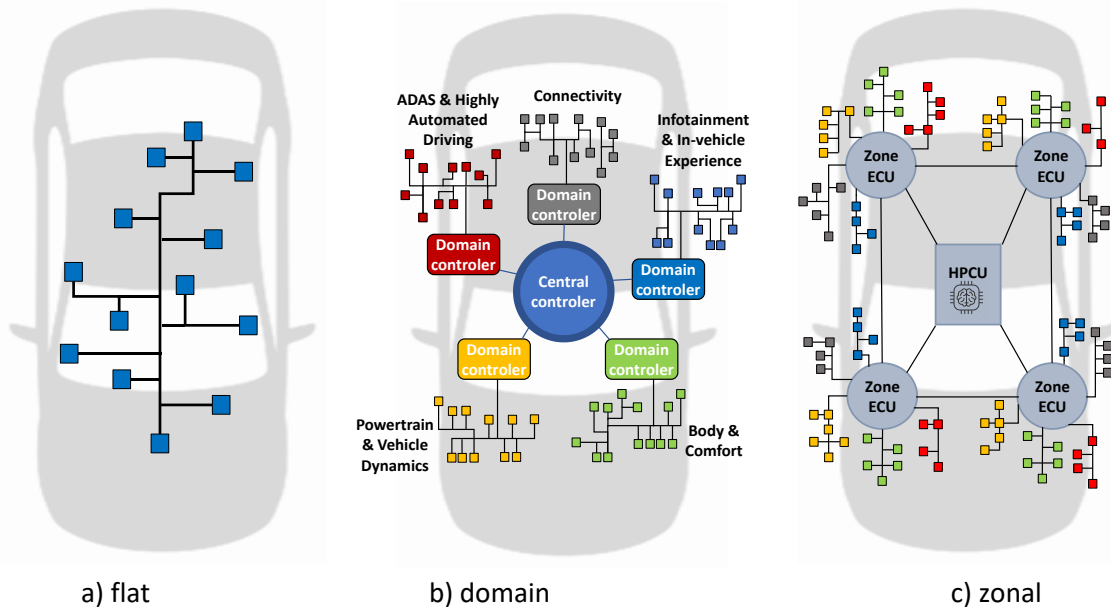
Figure 32: Evolution of vehicular E/E architectures
