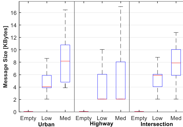
Figure 50: Message size at the output of the Autoware's perception module for different driving scenarios.
