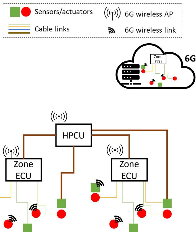
Figure 41: Integration of the 6G in-vehicle network with the 6G parent network.
